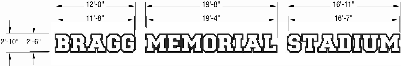
FOOTER DETAIL 1/8" = 1'-0"
