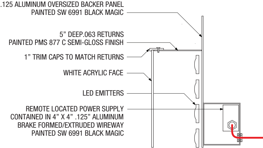
FACE ILLUMINATING SIGNAGE DETAIL NTS
